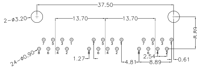
RECOMMENDED PCB LAYOUT VIEWED FROM COMPONENT SIDE
