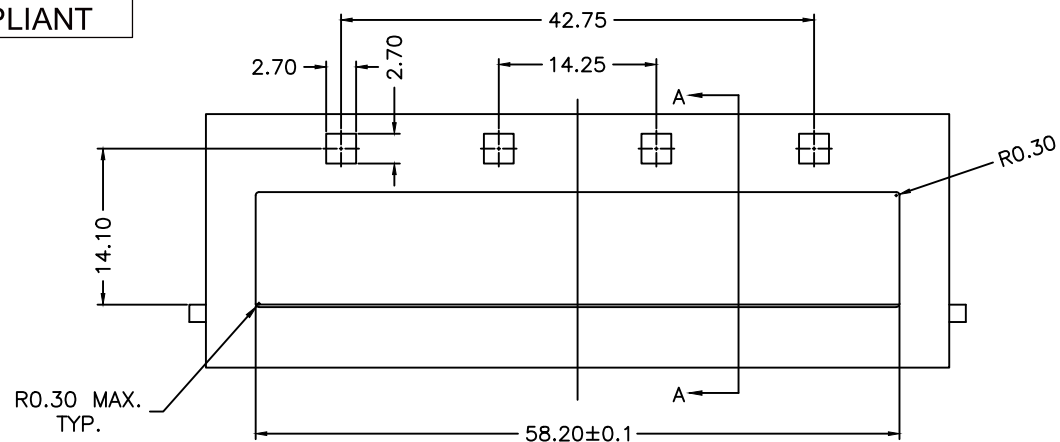
RECOMMENDED BEZEL DESIGN SINGLE SIDED APPLICATIONS
