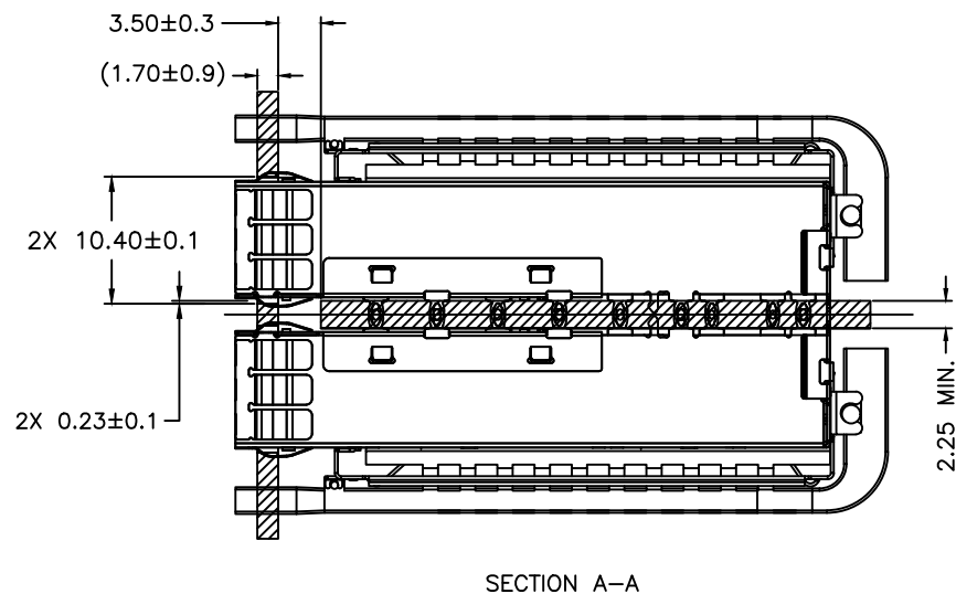
RECOMMENDED BEZEL DESIGN BELLY TO BELLY APPLICATIONS
