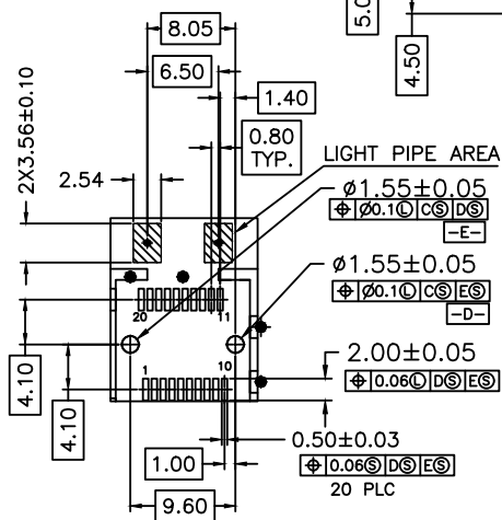
DETAIL H RECOMMENDED CONNECTOR LAYOUT 6X INDIVIDUALLY
