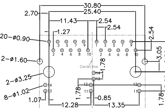
RECOMMENDED PCB LAYOUT VIEWED FROM COMPONENT SIDE
